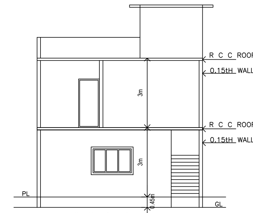
SECTION @ X-X
